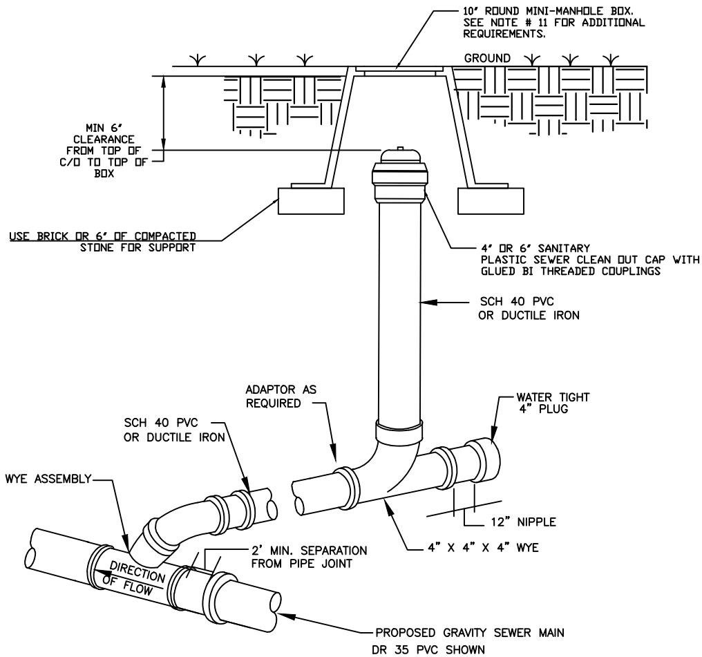
STANDARD SANITARY SEWER LATERAL WITH MINI-MANHOLE
