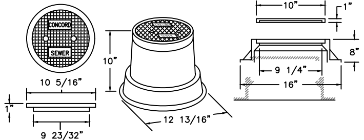
STANDARD SANITARY SEWER CLEANOUT WITH MINI-MANHOLE
