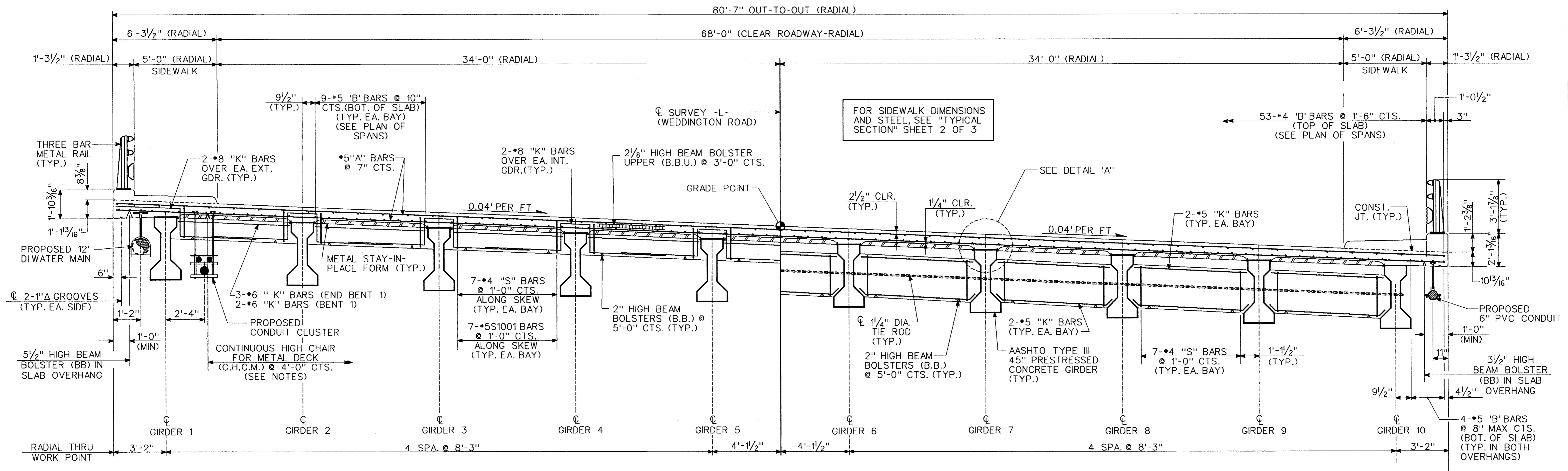
HALF SECTION AT END BENT 1 AND BENT 1 - SPAN A
