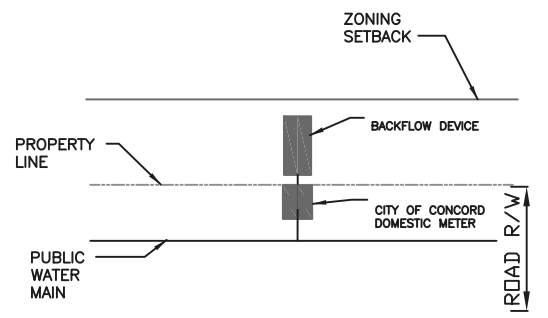
TYPICAL LOCATION REQUIREMENT N.T.S.
